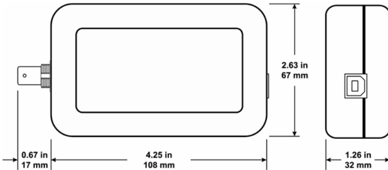
Figure 2 — USB22-CXB Dimensions
